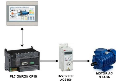
Gambar 1. Sistem Monitoring SCADA Variable Speed Drives
