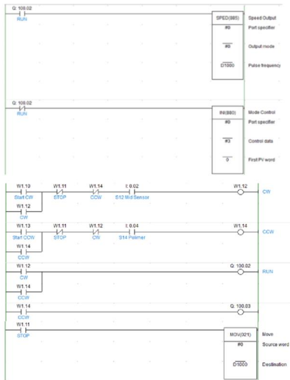
Gambar 5. Diagram Tangga Variable speed Drive
